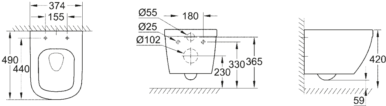
39 206 000 39 206 00H* Compact hangtoilet Triple Vortex
