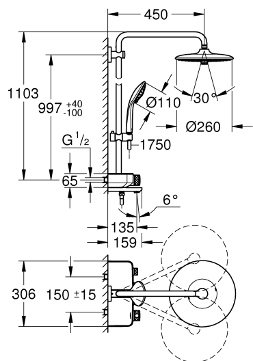
EUPHORIA SMARTCONTROL SYSTEM 260 MONO 26608000
