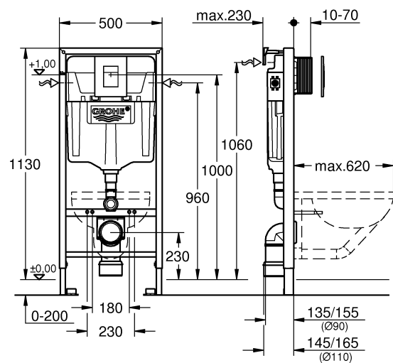
RAPID SL 3-IN-1 38772001
