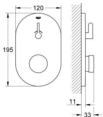
EUROSMART COSMOPOLITAN T 36321000
