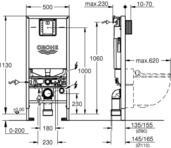
RAPID SLX 3-IN-1 39598000
