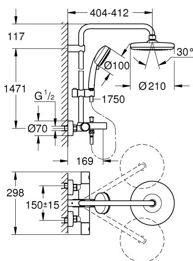
TEMPESTA COSMOPOLITAN SYSTEM 210 26223001
