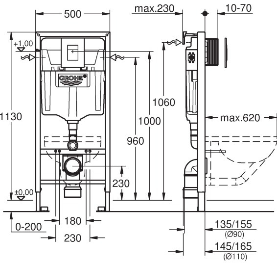
RAPID SL 3-IN-1 38772001
