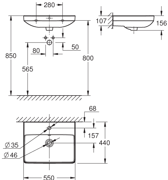
EURO CERAMIC 102430SH00
