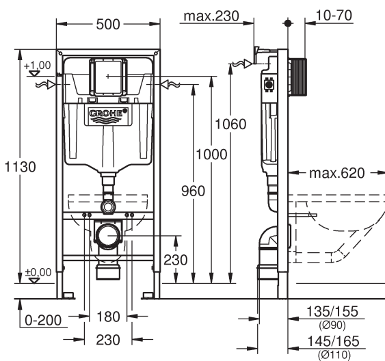
RAPID SL 2-IN-1 38536001
