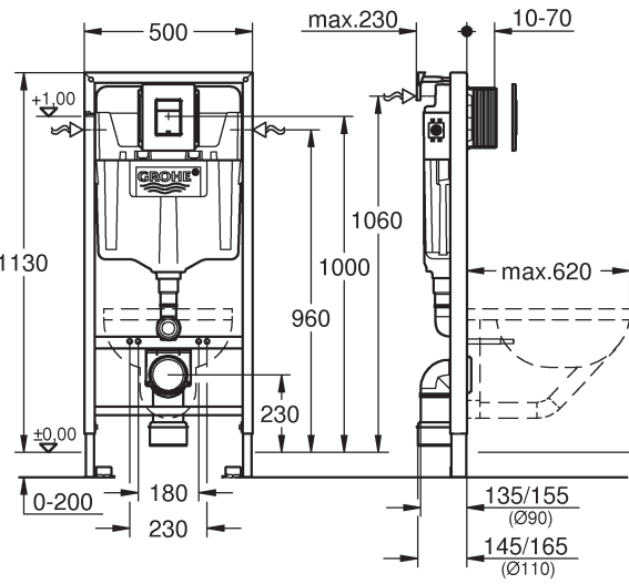
SOLIDO 3-IN-1 38811KF0
