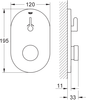
EUROSMART COSMOPOLITAN T 36321000
