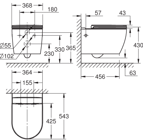
BAU CERAMIC 103860SH00
