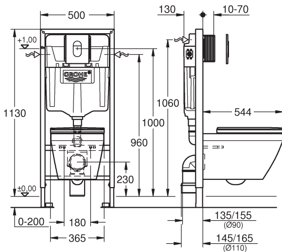
SOLIDO 5-IN-1 102514SH00
