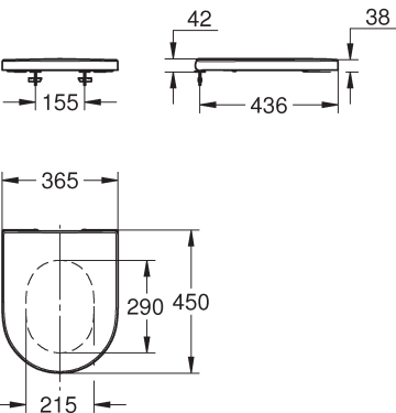
EURO CERAMIC 102501SH00
