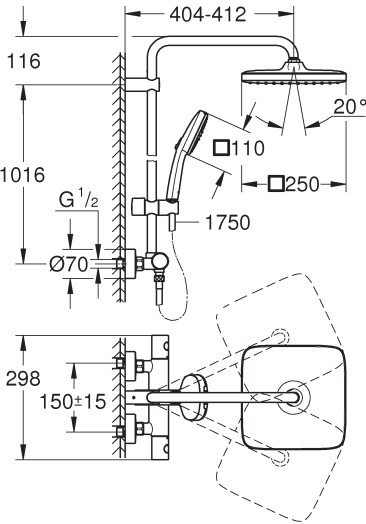
TEMPESTA SYSTEM 250 CUBE 26689001 / 266892431
