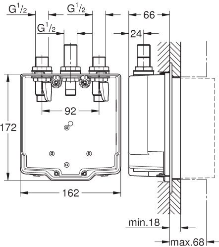
EUROSMART COSMOPOLITAN T 36322001
