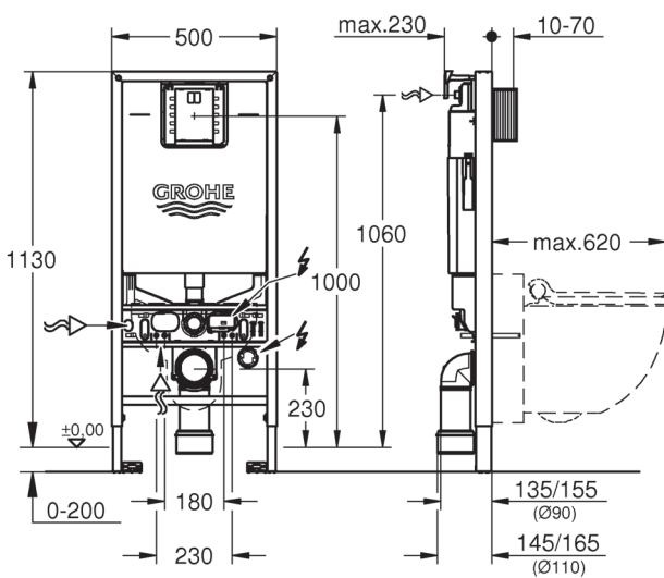
RAPID SLX 3-IN-1 39598000
