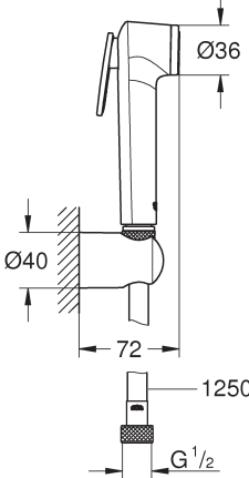
TEMPESTA-F TRIGGER SPRAY 30 1025302431
