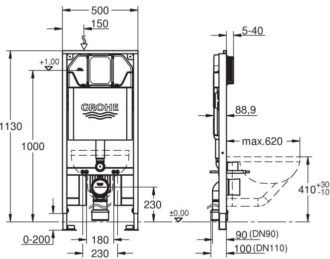
RAPID SL SLIM 39687000
