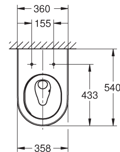
EURO CERAMIC 102501SH00
