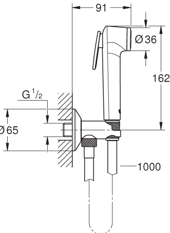
TEMPESTA-F TRIGGER SPRAY 30 26358000
