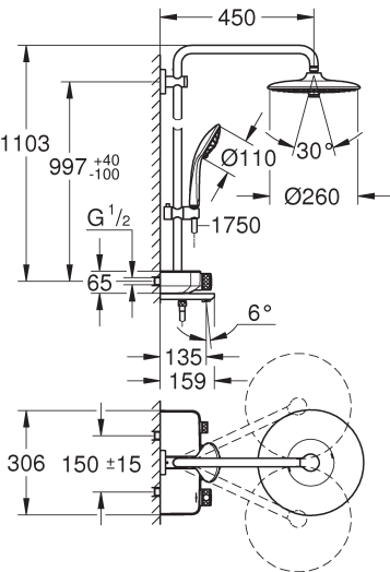
EUPHORIA SMARTCONTROL SYSTEM 260 26608000
