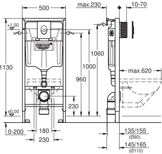
RAPID SL 3-IN-1 38722001
