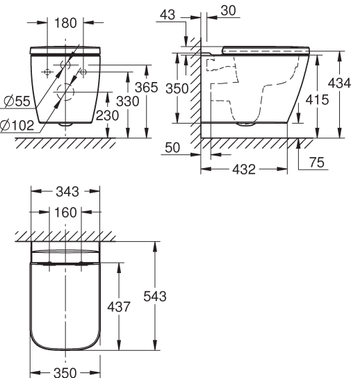
BAUEDGE CERAMIC 106740SH00
