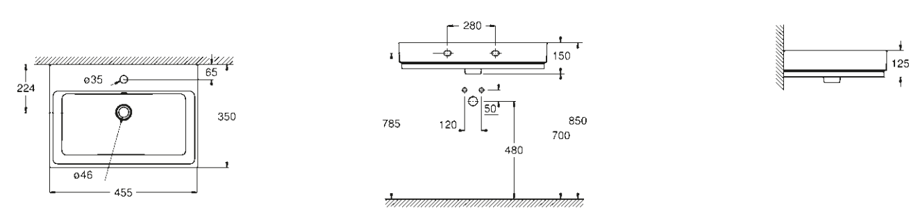
39 483 00H Handrinse basin 45 cm
