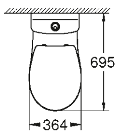
39 346 000 WC closed coupled combination: WC, rimless, vertical outlet (39 429 000) Cistern side inlet (39 437 000) Seat & cover soft close (39 493 000)
