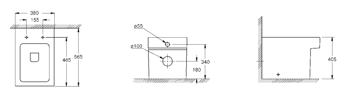
39 485 00H Floorstanding WC back to wall rimless
