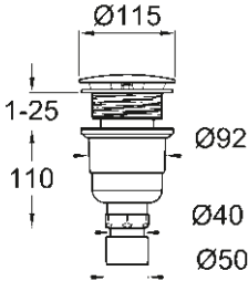
49 533 000* Waste set vertical for Universal shower trays
