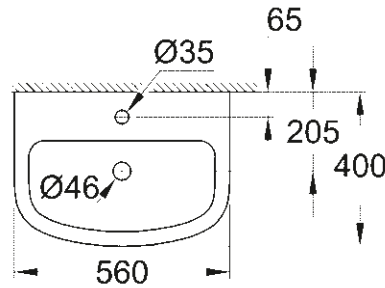
39 422 000 Drop in basin 55 cm
