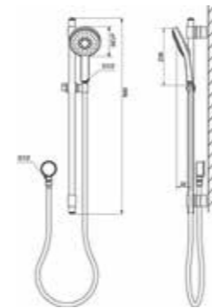
124 577 Shower rail set Power&Soul® Cosmopolitan 130
