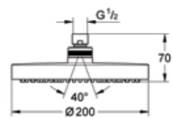
27 541 000 Overhead shower New Tempesta Cosmopolitan 200
