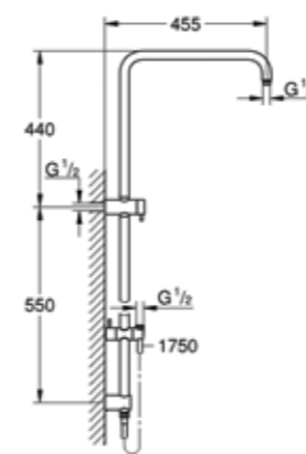
26 167 000 Shower system with diverter
