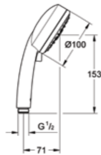
27 573 001 Hand shower New Tempesta Cosmopolitan 100
