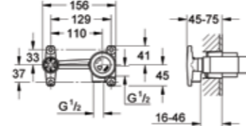
33 769 000 Single-lever mixer 1/2", concealed body
