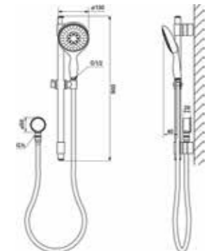
124 578 Shower rail set Power&Soul® 130
