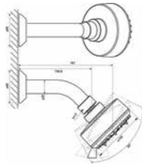
27 869 000 Overhead shower set New Tempesta Cosmopolitan 100 (Exclusive in ANZ*)
