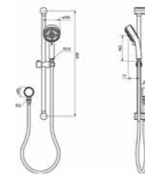
124 576 Shower rail set New Tempesta Cosmopolitan 100
