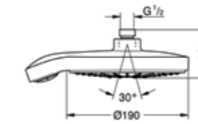
27 765 000 Overhead shower Power and Soul® Cosmopolitan 190
