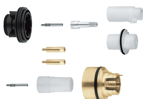
47 780 000 Extension set 27.5 mm for 36 458 000 / 36 459 000
