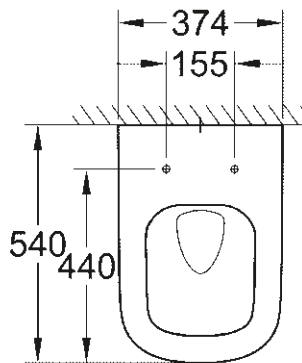
39 339 000 39 339 00H* Floorstanding WC back to wall rimless
