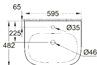
39 335 000 39 335 00H* Wall hung basin 60 cm
