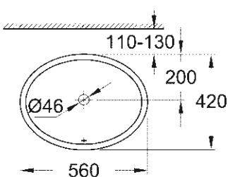
39 423 000 Undercounter basin 55 cm
