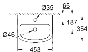
39 424 000 Handrinse basin 45 cm
