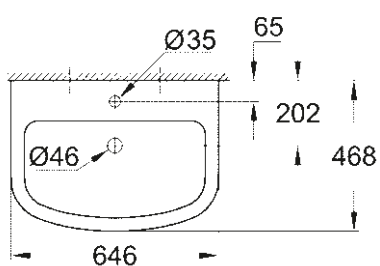
39 420 000 Wall hung basin 65 cm
