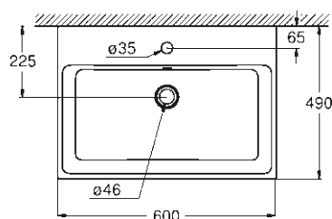
39 473 00H Wall hung basin 60 cm
