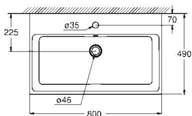
39 469 00H Wall hung basin 80 cm
