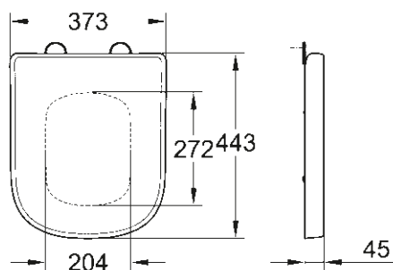
39 330 000 Seat & cover soft close quick release function 39 331 000 w/o soft close
