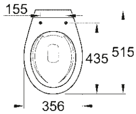
39 430 000 Floorstanding WC rimless
