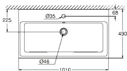
39 386 00H Wall hung basin 100 cm
