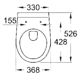
39 491 000 Wall hung WC open rim
