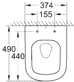
39 206 000 39 206 00H* Compact wall hung WC Triple Vortex
