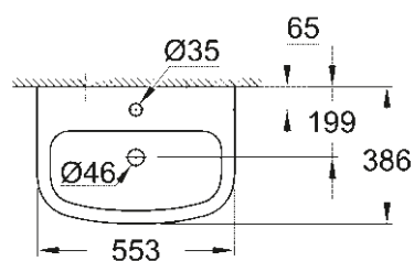
39 440 000 Wall hung basin 55 cm
