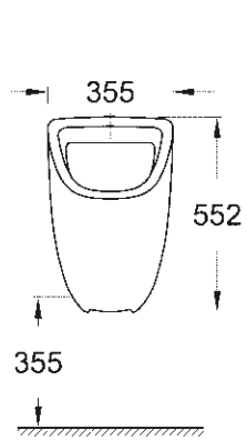
39 439 000 Urinal top inlet
