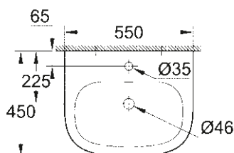
39 336 000 39 336 00H* Wall hung basin 55 cm
