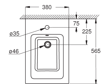
39 486 00H Wall hung bidet
