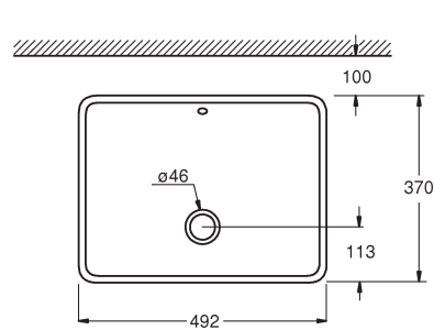
39 480 00H Undercounter basin 50 cm
