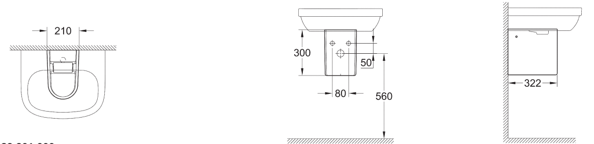
39 201 000 Semi pedestal for wash basins
