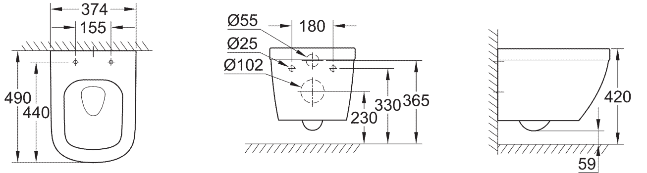
39 206 000 39 206 00H* Compact wall hung WC Triple Vortex
