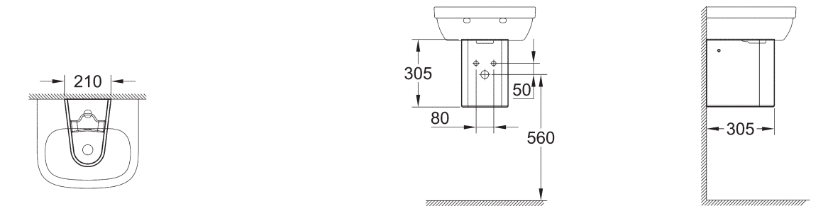
39 325 000 Semi pedestal for handrinse basin 45 cm
