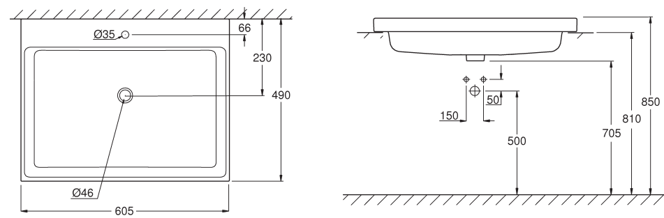
39 479 00H Drop-in basin 60 cm
