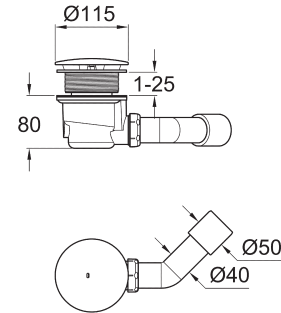
49 534 000* Waste set horizontal for Universal shower trays
