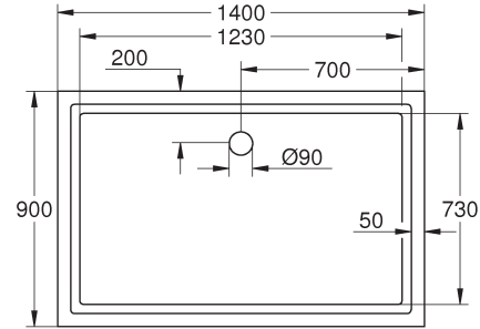
39 307 000* Universal shower tray 90 cm x 140 cm
