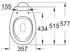
39 431 000 Floorstanding WC rimless
