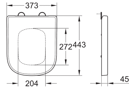
39 330 000 Seat & cover soft close quick release function 39 331 000 w/o soft close
