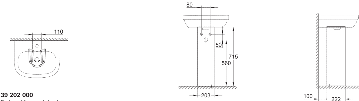
39 202 000 Pedestal for wash basins
