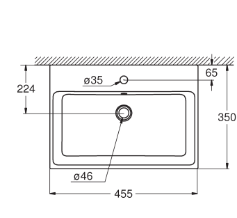
39 483 00H Handrinse basin 45 cm
