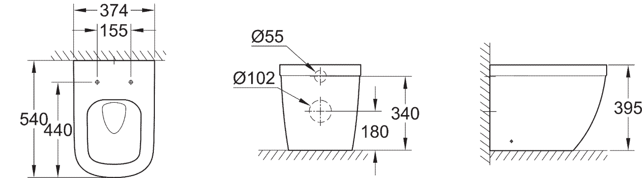
39 339 000 39 339 00H* Floorstanding WC back to wall rimless
