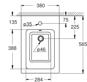
39 487 00H Floorstanding bidet
