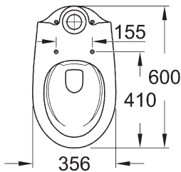
39 349 000 Floorstanding WC for closed coupled combination rimless, horizontal outlet 39 428 000 boxed rim
