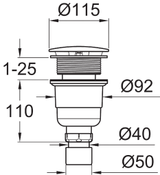
49 533 000* Waste set vertical for Universal shower trays
