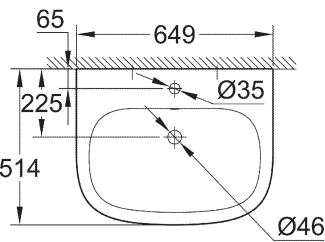
39 323 000 39 323 00H* Wall hung basin 65 cm
