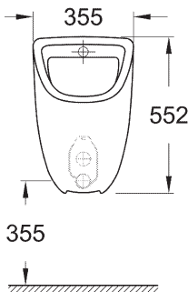
39 438 000 Urinal concealed inlet
