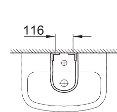
39 426 000 Semi pedestal for wash basins
