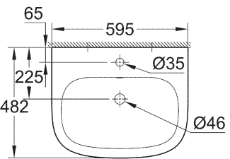
39 335 000 39 335 00H* Wall hung basin 60 cm
