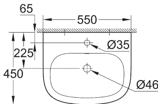
39 336 000 39 336 00H* Wall hung basin 55 cm
