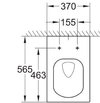
39 244 00H Wall hung WC Triple Vortex
