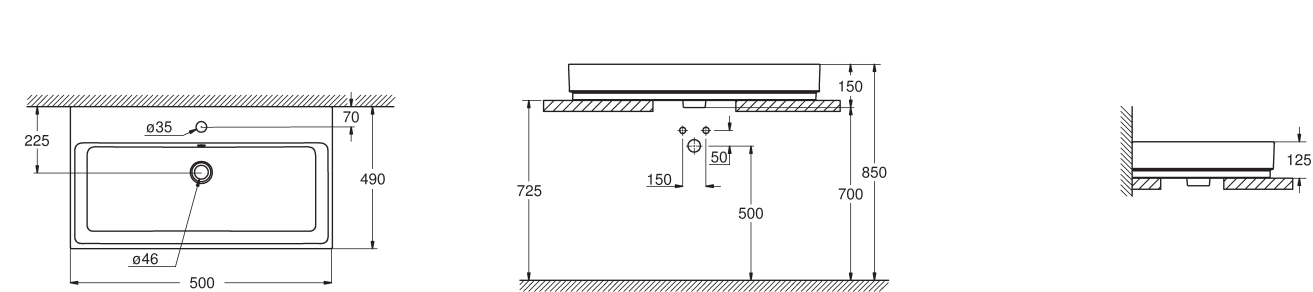
39 478 00H Countertop basin 50 cm
