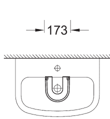
39 425 000 Pedestal for wash basins
