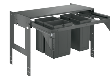
40 983 000 Extractible waste system, 90 cm cabinet, 2 x 8 + 11 liter waste bins
