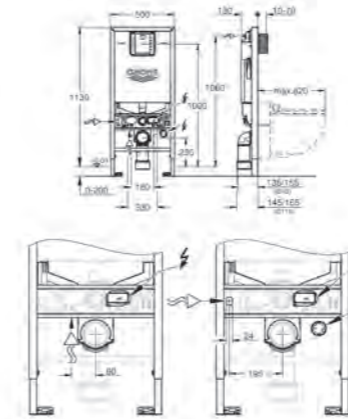
39 596 000 Inwall Cistern Rapid SLX Installation System Suitable for Sensia Arena and wall hung pans WELS 4 Stars, 4.5/3ltrs/min
