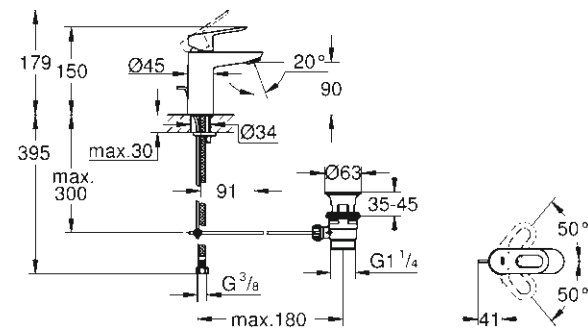
23 335 000 S-Size, OHM with pop up waste set
