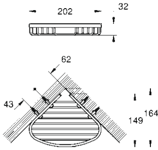
40 664 001 Filling basket, small
