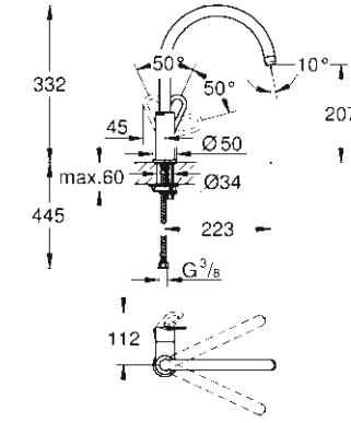
31 368 000 GROHE BauLoop Kitchen sink mixer
