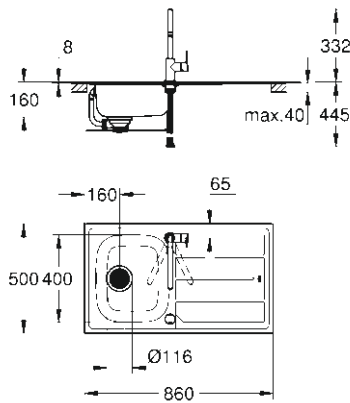
31 562 SD0 Bau Sink Bundle Kitchen Faucet and Sink Bundle consisting of: Stainless steel kitchen sink K200 Single lever sink mixer BauEdge with swivel spout
