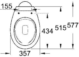
39 431 000 Floorstanding WC, wash down, vertical outlet
