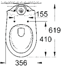
39 428 000 Floorstanding WC close coupled, wash down, horizontal outlet
