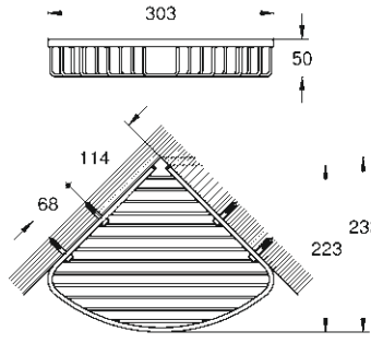
40 663 001 Large corner basket
