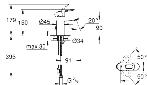
23 336 000 S-Size, OHM with retractable chain
