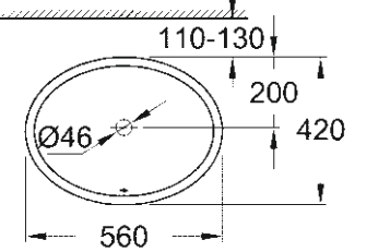
39 423 000 Undercounter basin, 55 cm
