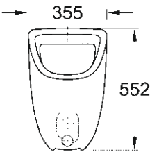
39 439 000 Urinal top inlet
