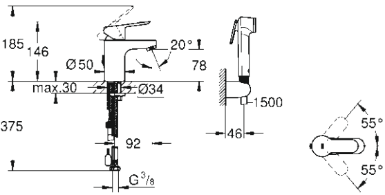
23 757 000 S-Size, OHM with multi-functional shower
