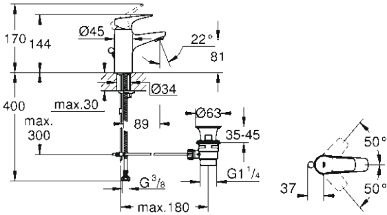
23 751 000 S-Size, OHM with pop up waste set
