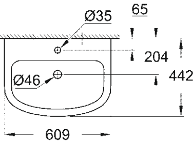
39 421 000 Wall hung basin, 60 cm
