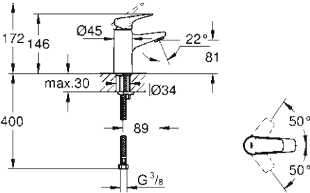
23 752 000 S-Size, OHM with smooth body
