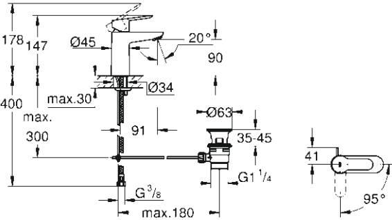
23 559 000 S-Size, OHM Longlife ES with pop up waste set
