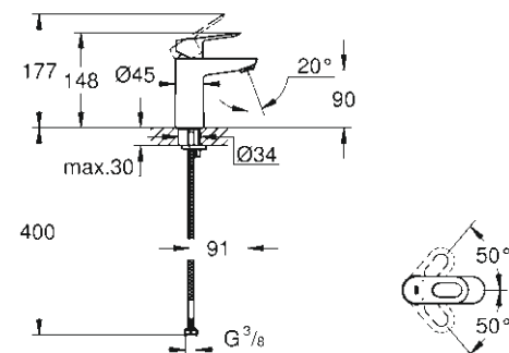
23 337 000 S-Size, OHM with smooth body
