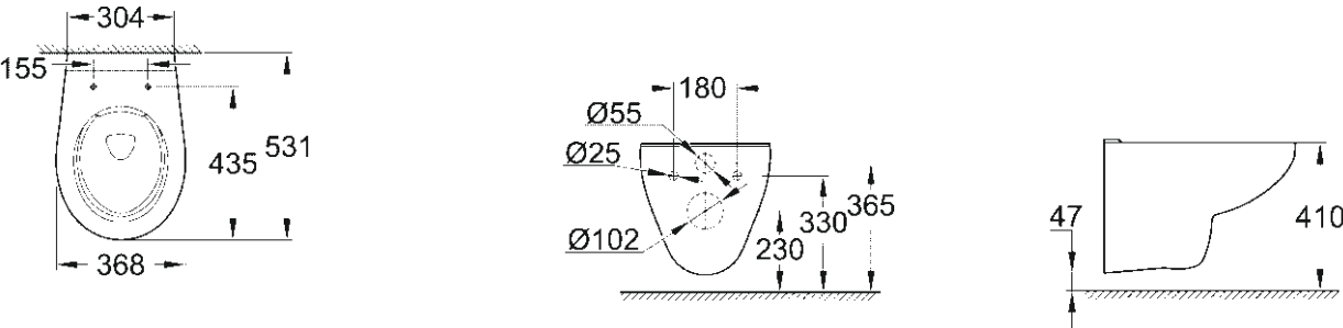
39 427 000 Wall hung WC, wash down
