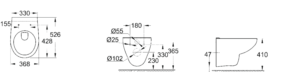
39 491 000 Wall hung WC, open rim
