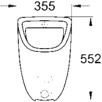
39 438 000 Urinal concealed inlet
