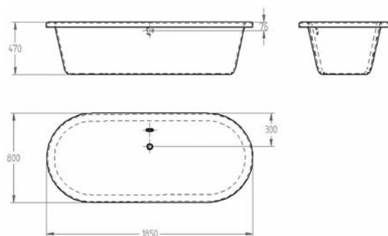
39 151 000 Bath tub - drop-in 180 x 80 Alpine White
