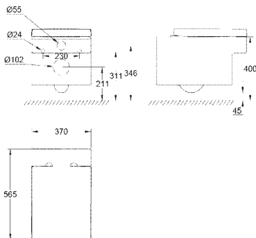
39 244 000 WC - Wall hung Alpine White
