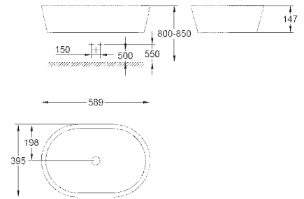
39 122 001 Vessel basin 60 Alpine White
