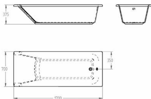
39 150 000 Bath tub - drop-in 170 x 70 Alpine White
