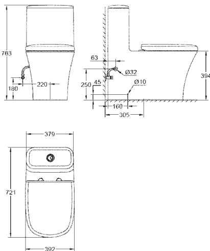
39 310 000 Floorstanding 1 PC toilet Alpine White
