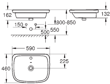
39 276 000 Counter basin built-in 60 Alpine White
