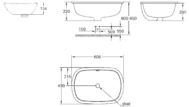
39 125 001 Washbasin under-counter 60 Alpine White
