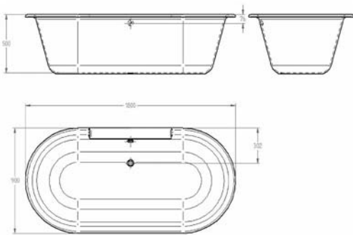
39 154 000 Bath tub - drop-in 180 x 90 Alpine White
