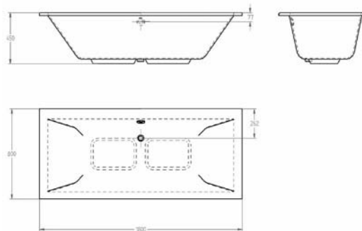
39 159 000 Bath tub - drop-in 180 x 80 Alpine White
