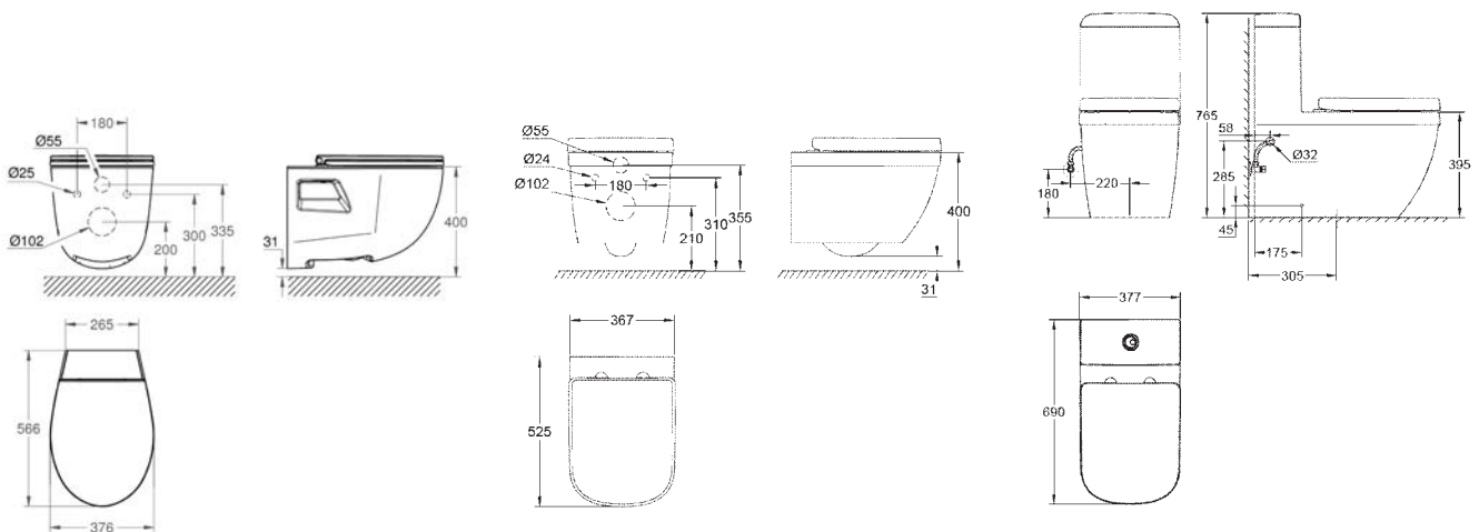
39 126 001 WC - Wall hung Alpine White
