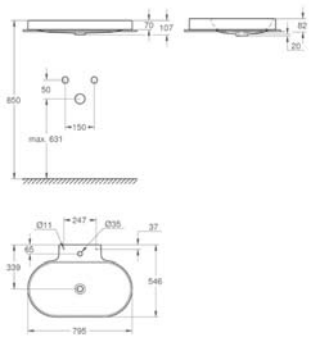
39 070 001 Counter basin w/o overflow 78 Alpine White
