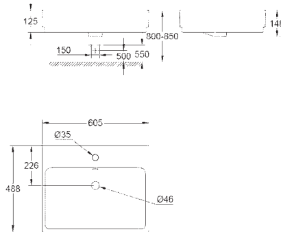
39 234 000 Counter basin 60 Alpine White
