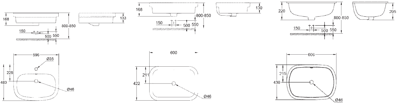
39 198 000 Counter basin 60 Alpine White
