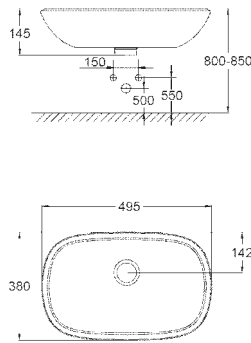
39 216 000 Vessel basin 50 Alpine White
