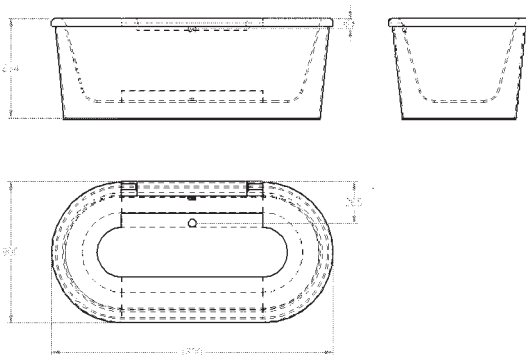
39 322 000 Surround for 39154000 Alpine White
