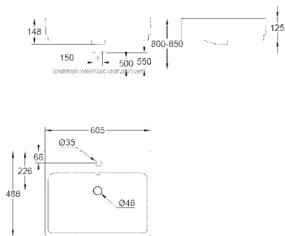
39 231 000 Washbasin wall hung 60 Alpine White
