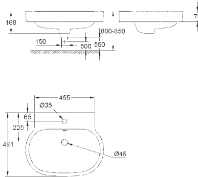
39 291 000 Counter basin 60 Alpine White
