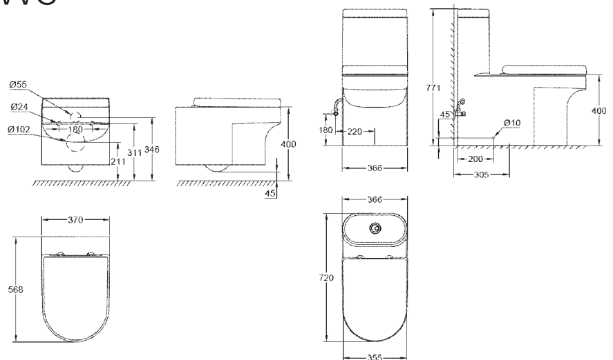
39 296 000 WC - Wall hung Alpine White
