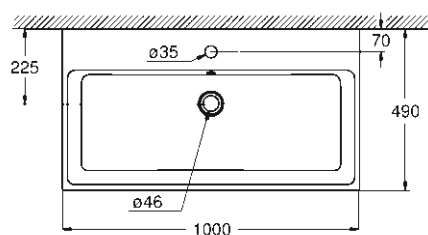
39 475 00H / 634133.060
