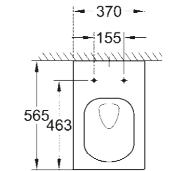
39 244 00H Wall hung WC Triple Vortex
