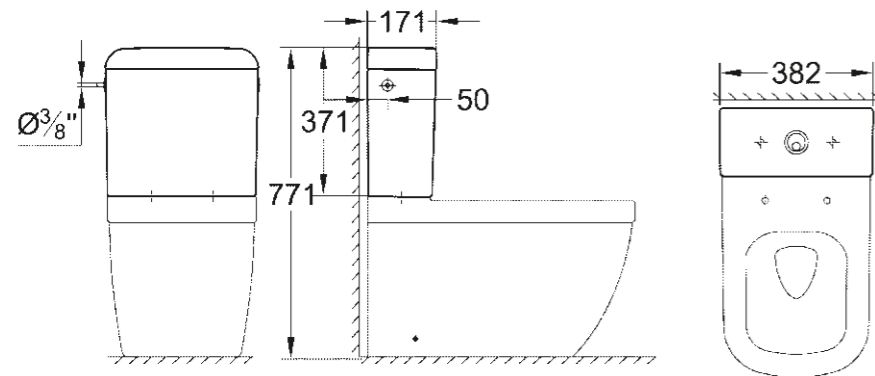
39 531 000 Cistern side and back inlet, NF
