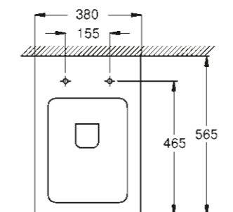
39 485 00H Floorstanding WC back to wall rimless
