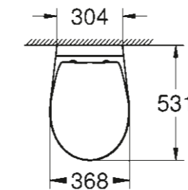
39 351 000 Wall hung WC rimless Seat & cover soft close Quick release function
