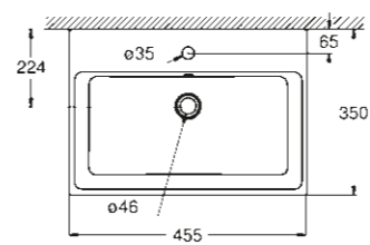
39 483 00H Handrinse basin 45 cm
